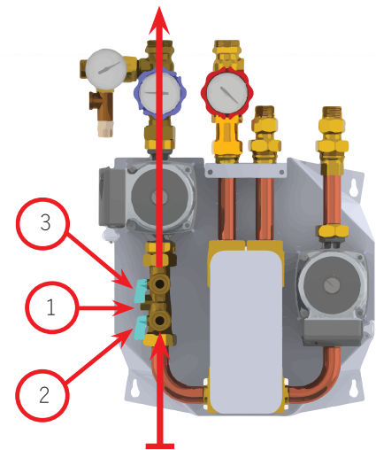
Figure 4.4-1: Fill port flow connections
