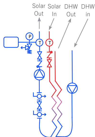
Figure 2.0.-2: HPAK Hydraulic
