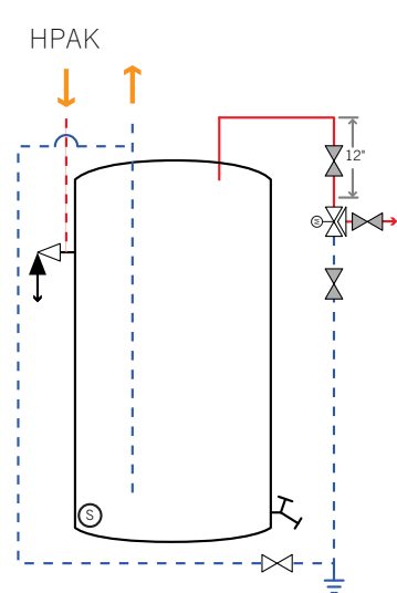
Figure 3.1-1: Single Standard Tank
