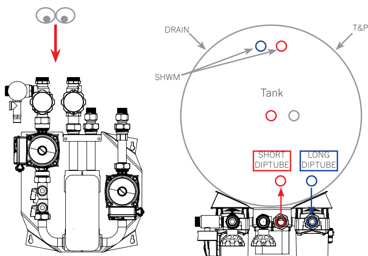
Figure 2.1.-1: HPAK and Tank Connections
