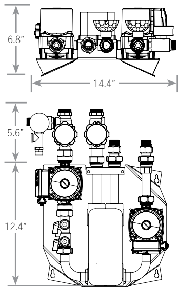
Figure 1B-1: HPAK Dimensions
