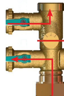
Figure 1.6.4.-2: Drain Fitting Open (Fluid Servicing)
