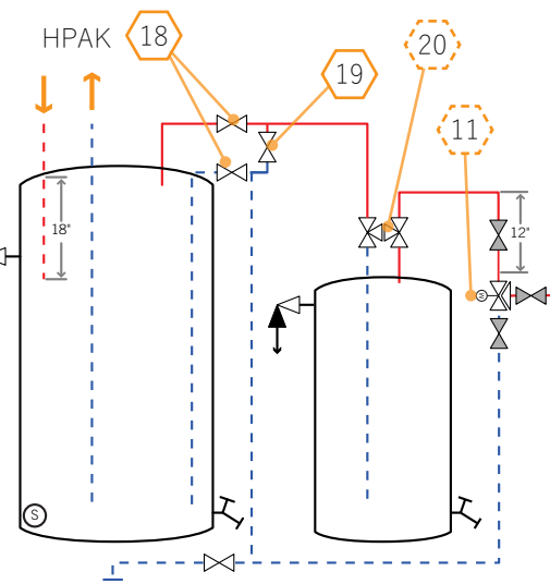
Figure 3.1-3: Dual Tank: Gas Backup
