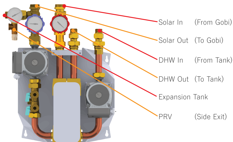
Figure 2.0.-1: HPAK Connections
