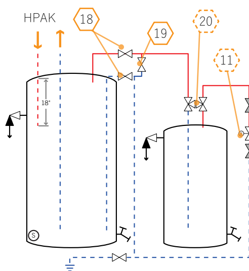
Figure 3.1-2: Dual Tank: Electric Backup
