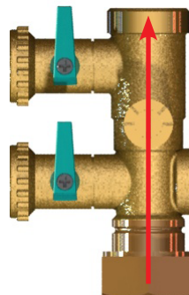
Figure 1.6.4.-1: Drain Fitting Closed (Operation Position)
