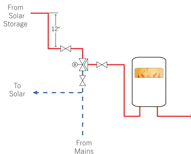
Figure 3.1-4: Flow Thru Connection
